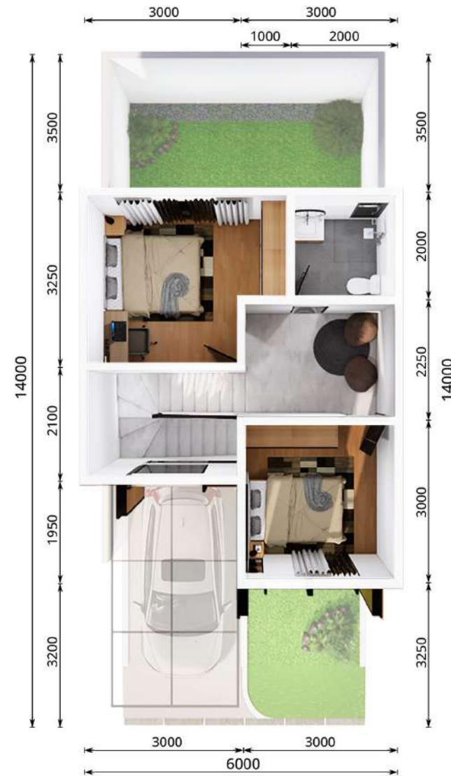
2nd Floor
